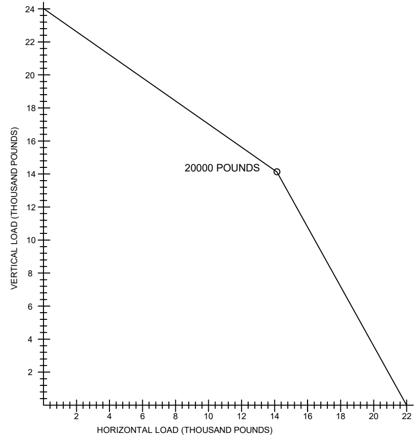
FIGURE 1 SEISMIC RATINGS (ATTACHMENT TO CONCRETE)
